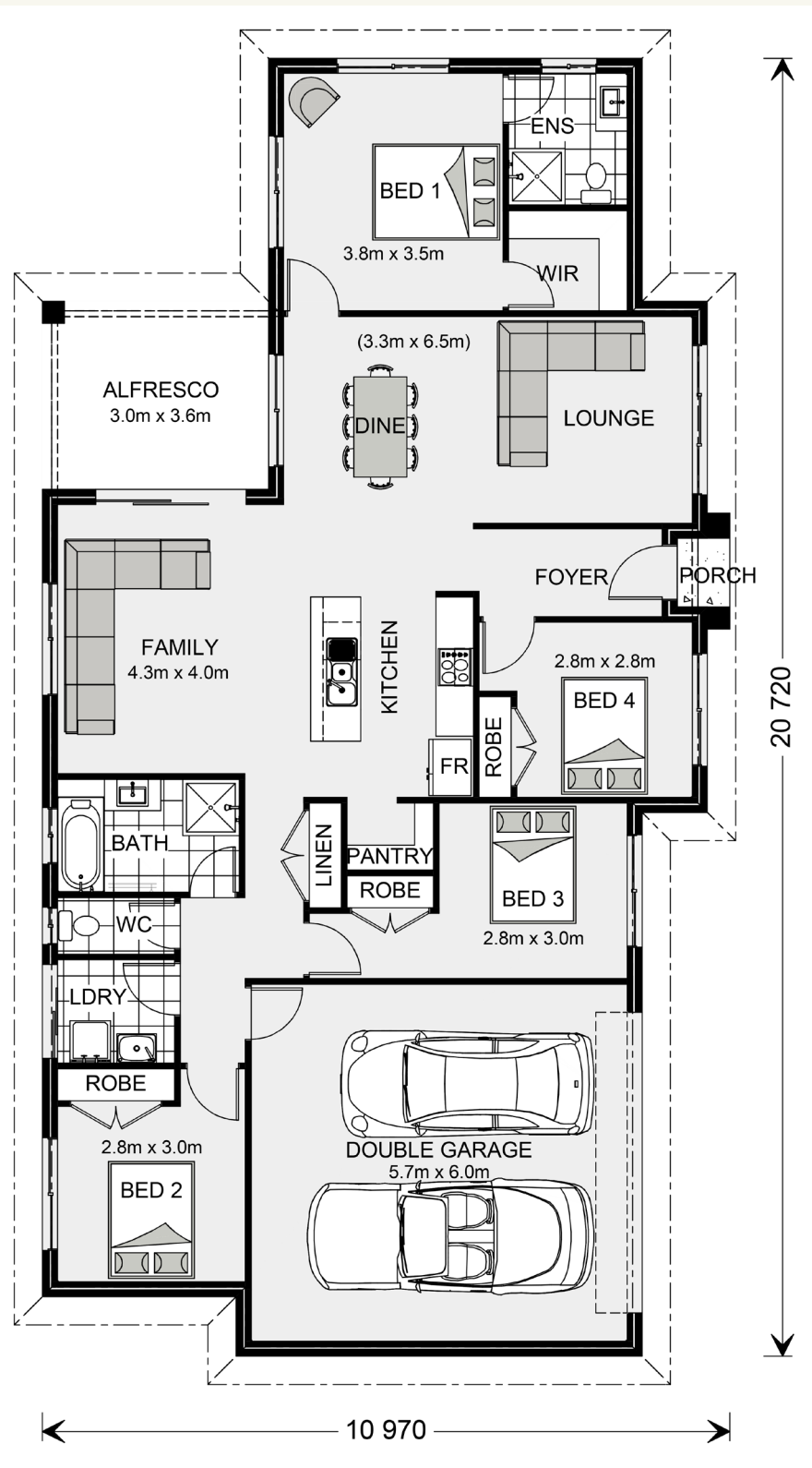
Wishart 190 Classic facade floorplan
